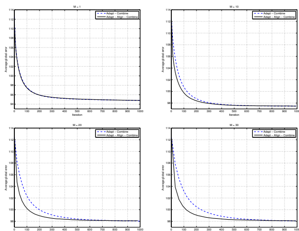
Fig. 2. Convergence comparison
